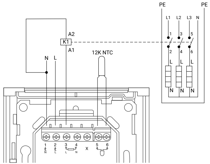
K1: contactor with integral suppression device
